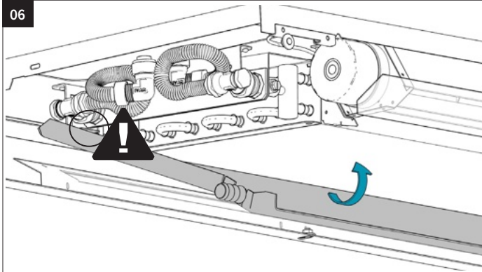
Install the condensate trap.
