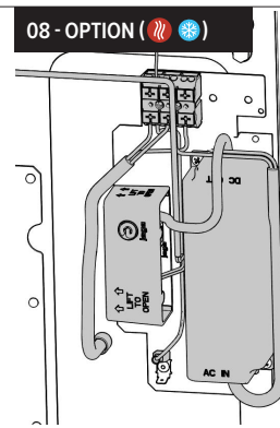
Connection to 230 VAC with waterproof power and cable gland.
