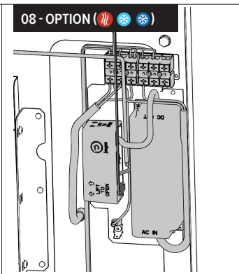
230 VAC connection with watertight power supply and pre-assembled condensate pump with breaker point (class I device).
