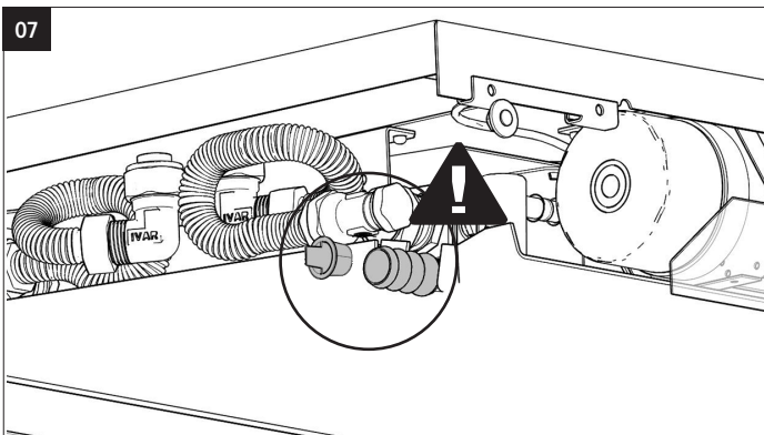
Non-condensing cooling - close the drain nipple of the condensate trap (Ø2cm).
