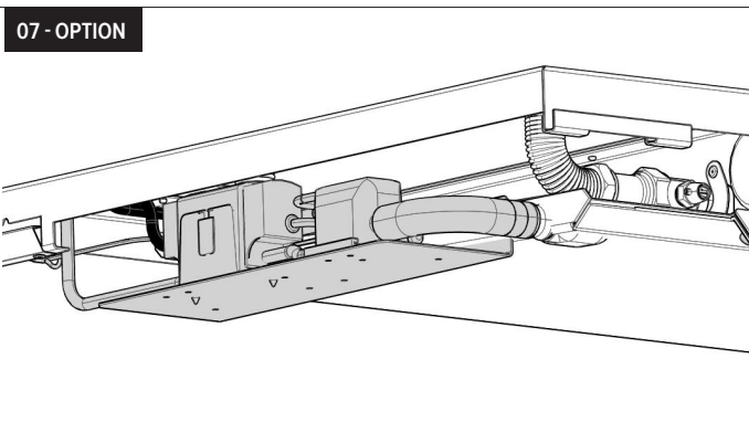
Condensing cooling - pre-assembled condensate pump with breaker point (class I device).
