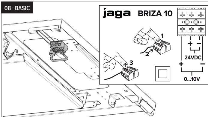
24 VDC connection with external control.
